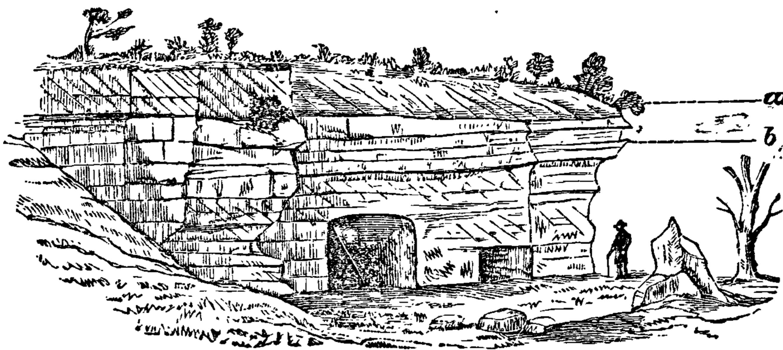
Fig. 91. Quarry at Yatton Keynell, near Corsham, a Forest Marble. Fissile shelly oolite, resting obliquely on the Great Oolite; 4 feet. b Great Oolite (upper zone). Regularly bedded massive shelly limestone; 7 feet. c Great Oolite (lower zone). Shelly oolite, full of false bedding. The upper part coarse; the lower affording very fine building stone, which is followed underground; 16 feet.
